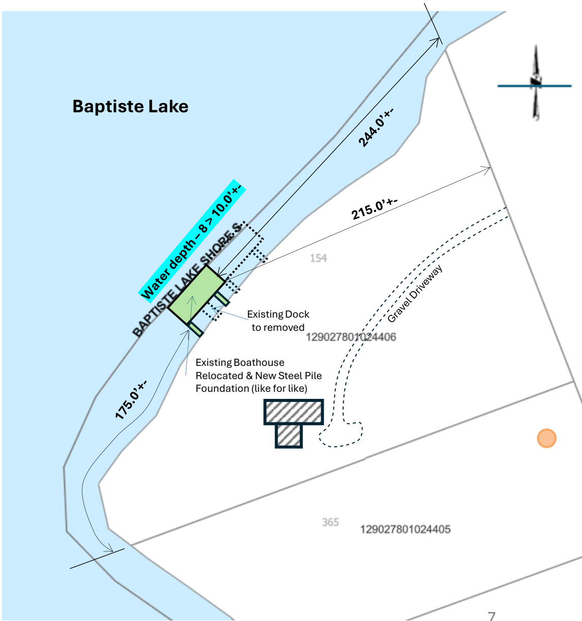
Site Plan & Pirate-ship Boathouse Proposed Location
