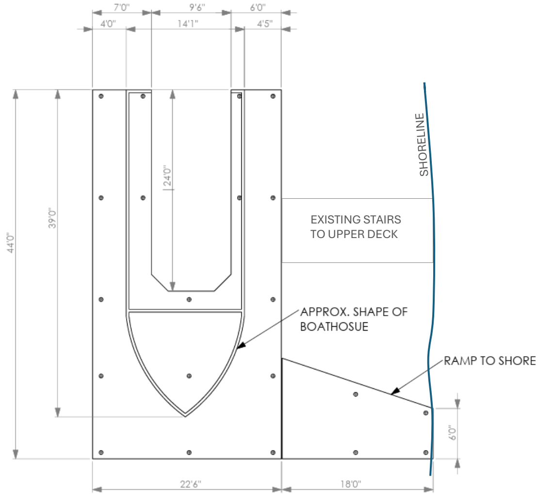
Existing Boathouse/Dock Layout
